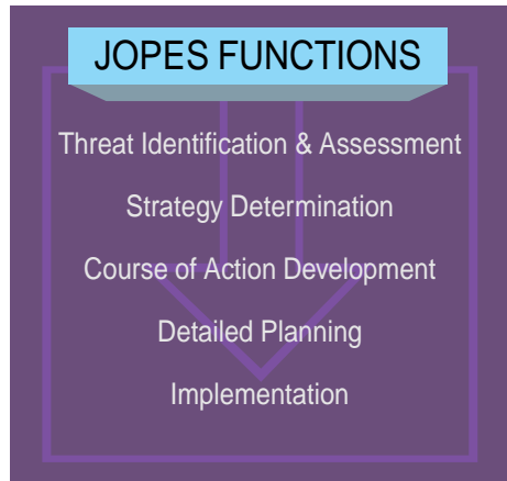
Figure I-6. JOPES Functions
